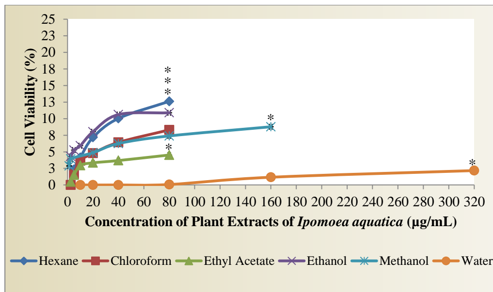
Figure 4.6: Antiviral activity of Ipomoea aquatica extracts at different concentrations against CHIKV in 72 hour post-inoculation antiviral assay. *Significant differences at p < 0.05 among different concentrations using One-way ANOVA test; Multiplicity of infection = 1
