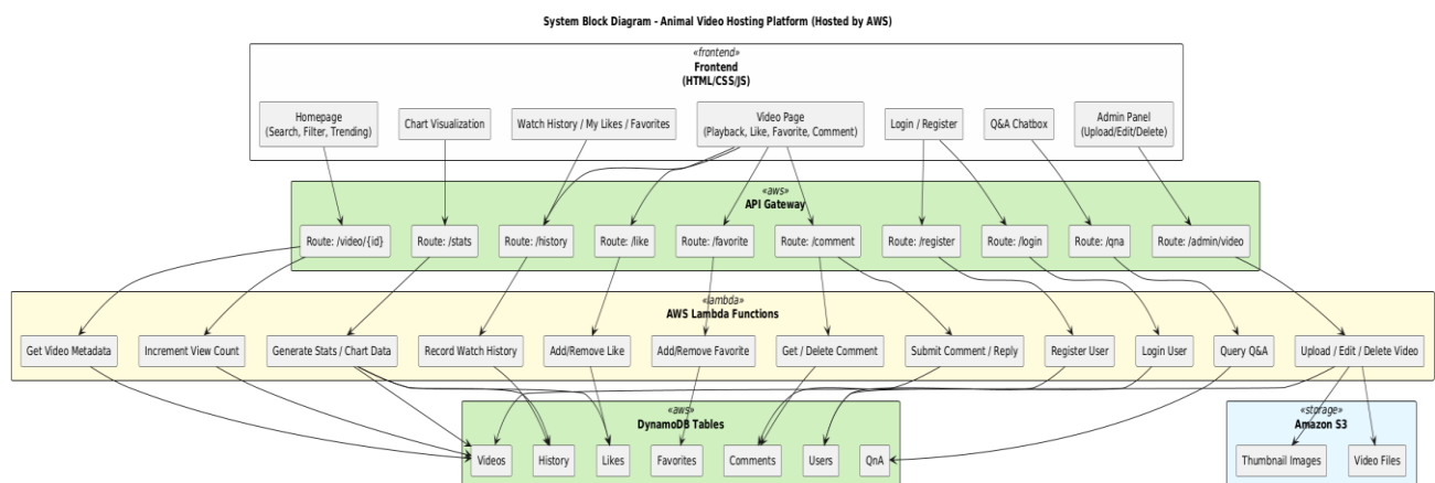
Figure 4.1.1 System Block Diagram of Animal Video Hosted By AWS
