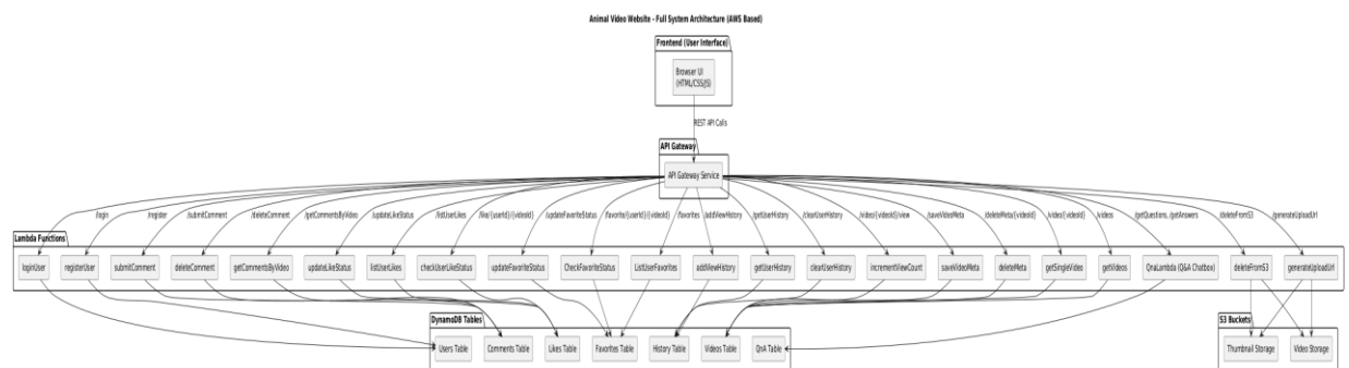
Figure 3.1.1 System Architecture Diagram of Animal Video Hosted by AWS
