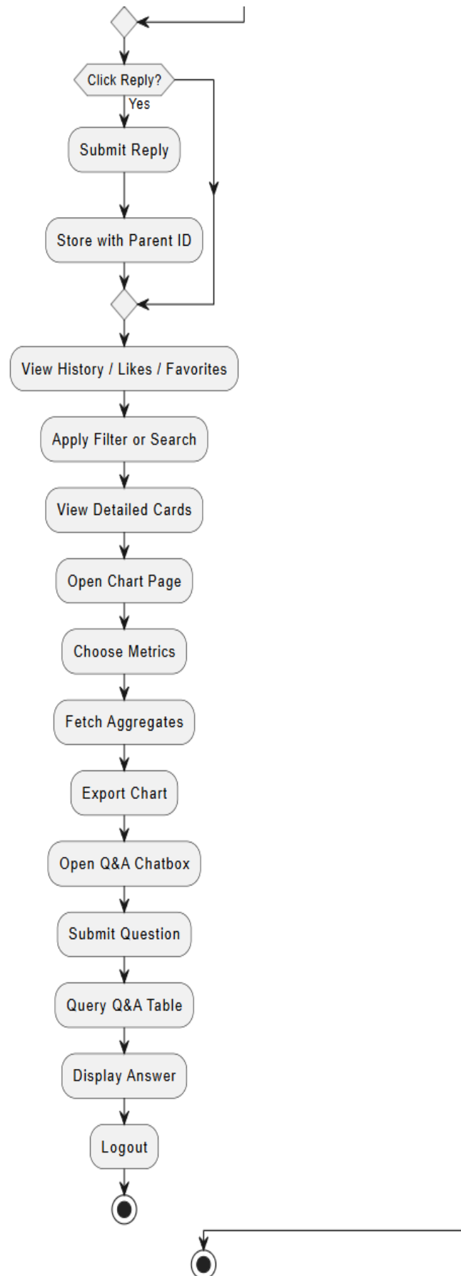
Figure 3.1.3 Activity Diagram of Animal Video Hosted By AWS
