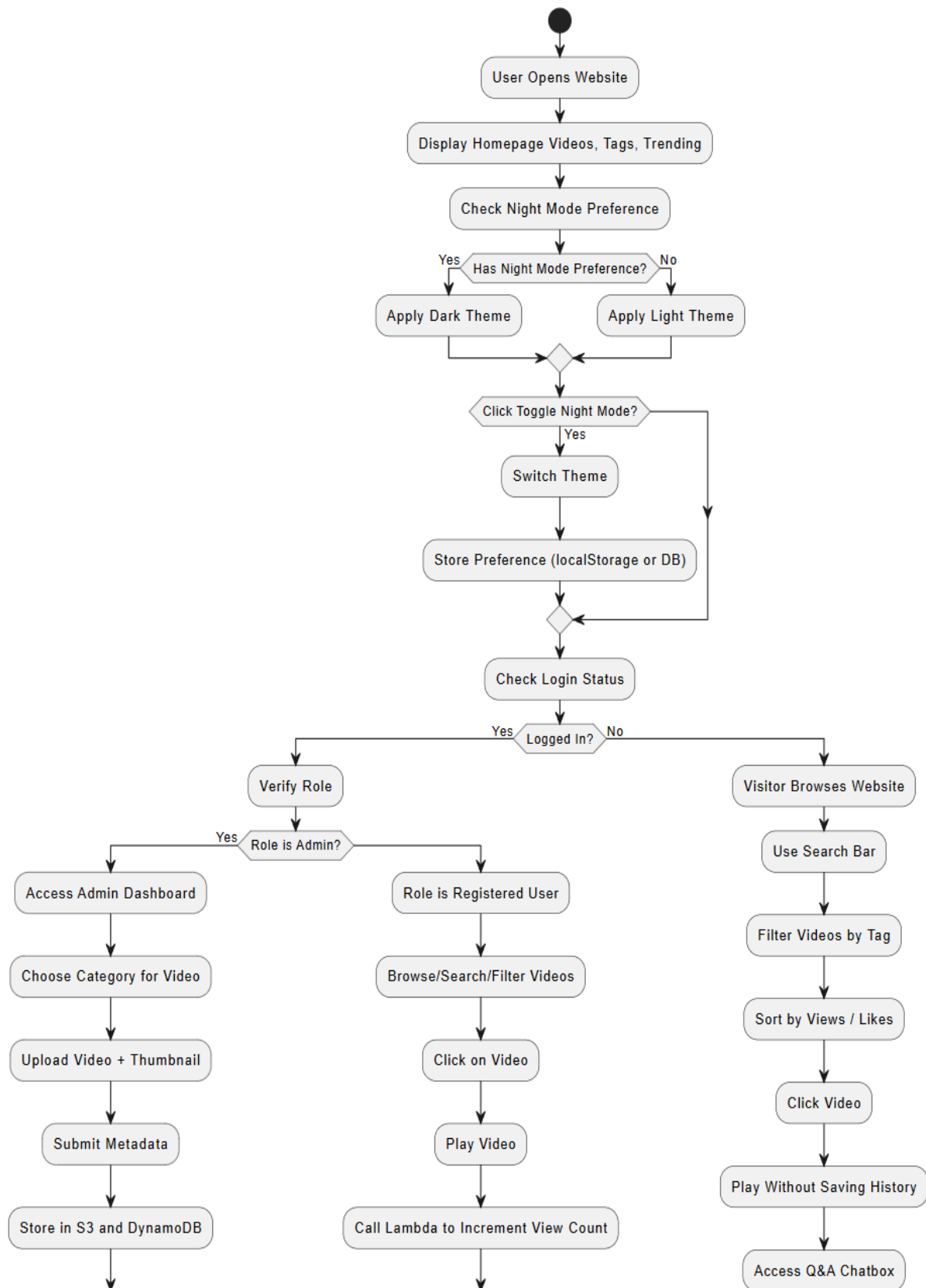
Animal Video Hosted By AWS Activity Diagram
