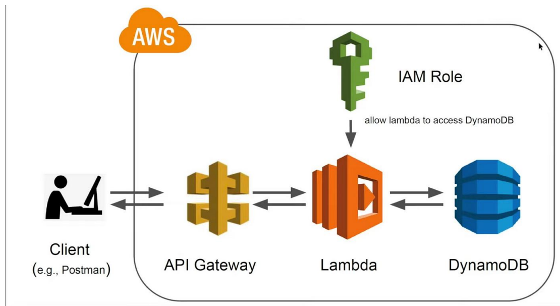
Figure 5.3.1 AWS Lambda, DynamoDB and API Gateway Setup
